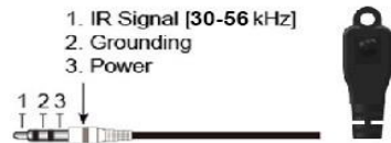
IR Receiver
